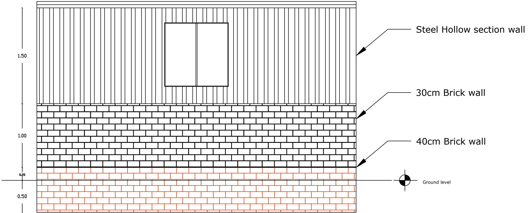
Side Elevation
